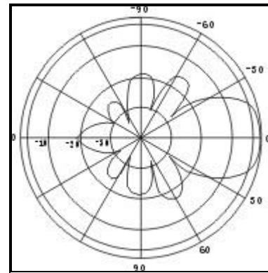
Vertical Plane
