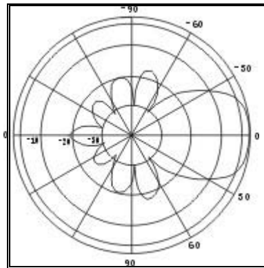
Horizontal Plane
