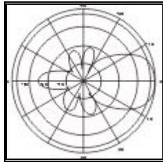
Horizontal Plane
